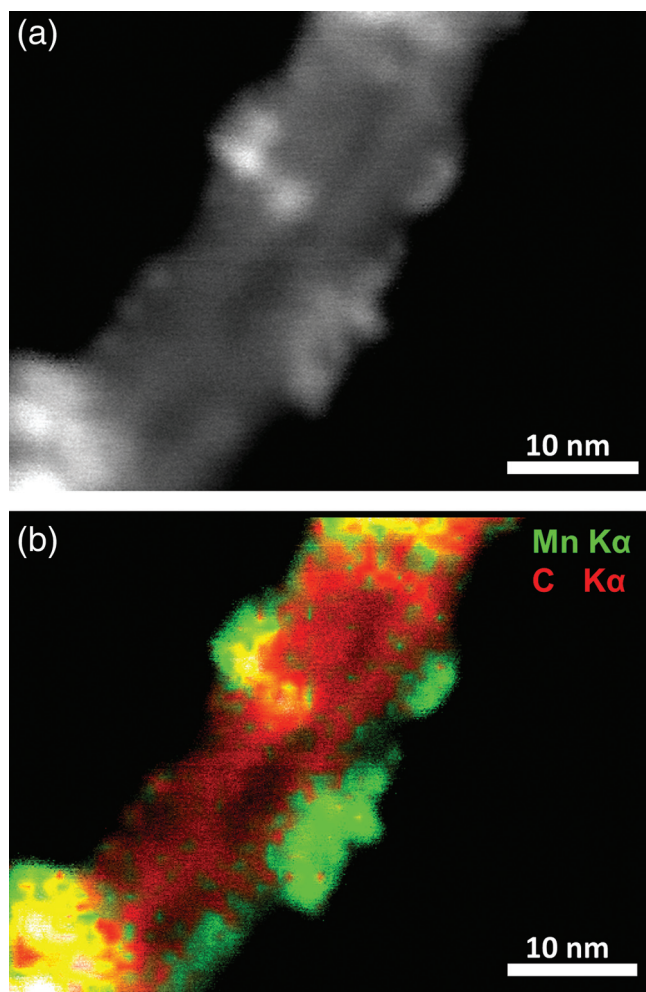
Figure 4. a) Z contrast HAADF-STEM image of \text{Mn}_4 -MWNT hybrid 2. b) STEM-EDS elemental mapping performed over the area represented in (a) showing excellent agreement between the Mn distribution and the bright spots grafted to the nanotube.
