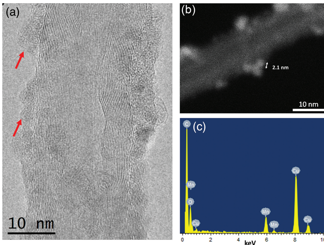
Figure 3. a) HRTEM images of 2 displaying the grafting of the Mn 4 complex (indicated by the arrows) on the negatively charged MWNTs. b) Z-contrast HAADF-STEM image showing the distribution of the clusters along the nanotubes (brighter spots) and their size (2.1 nm). c) Local area EDS spectrum confirming the presence of Mn on the MWNTs. Again, the Cu signal is attributed to the TEM grid.
