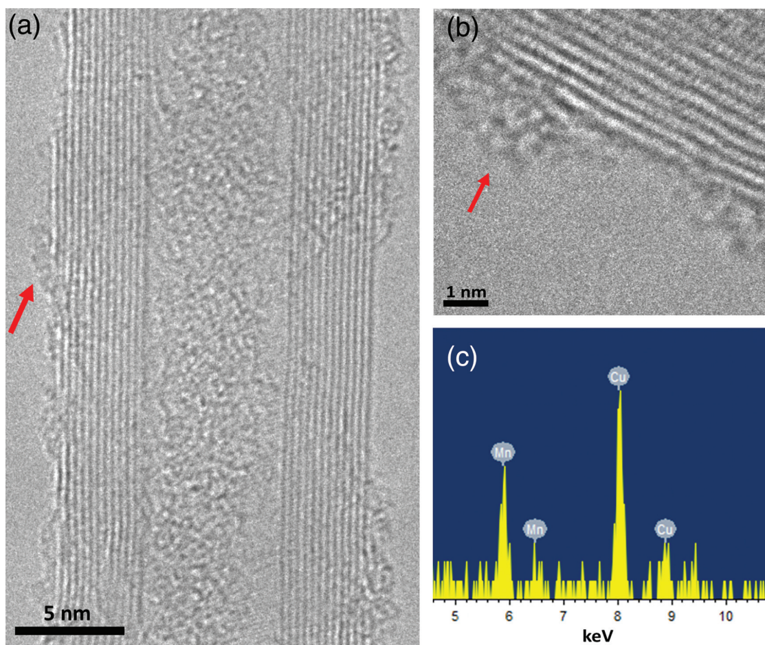
Figure 2. a,b) HRTEM images of 1 displaying the grafting of the \text{Mn}_4 complex (indicated by the arrows) on the surface of prefunctionalized MWNTs. The multiwalled structure of the CNTs can also be seen. c) EDS spectrum acquired from a single decorated MWNT like the one shown in (a), which confirms the presence of Mn. The Cu signal can be attributed to the TEM grid.
