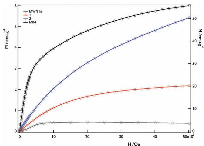
Figure 6. Isothermal field dependence of the magnetization of purified MWNTs (grey), \text{Mn}_4 -MWNTs hybrids 1 (red) and 2 (blue), and nongrafted \text{Mn}_4 complex (black). Solid lines are a guide to the eye.
