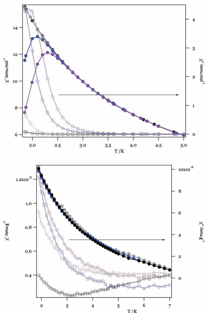
Figure 7. AC susceptibility of the hybrid 2 (top) and the pristine \text{Mn}_4 complex (bottom) collected in the 1 (black), 10 (grey), 110 (blue), and 333 Hz (purple) range. In-phase susceptibility and out-of-phase signals are represented by filled and empty symbols, respectively. Solid lines are a guide for the eye.
