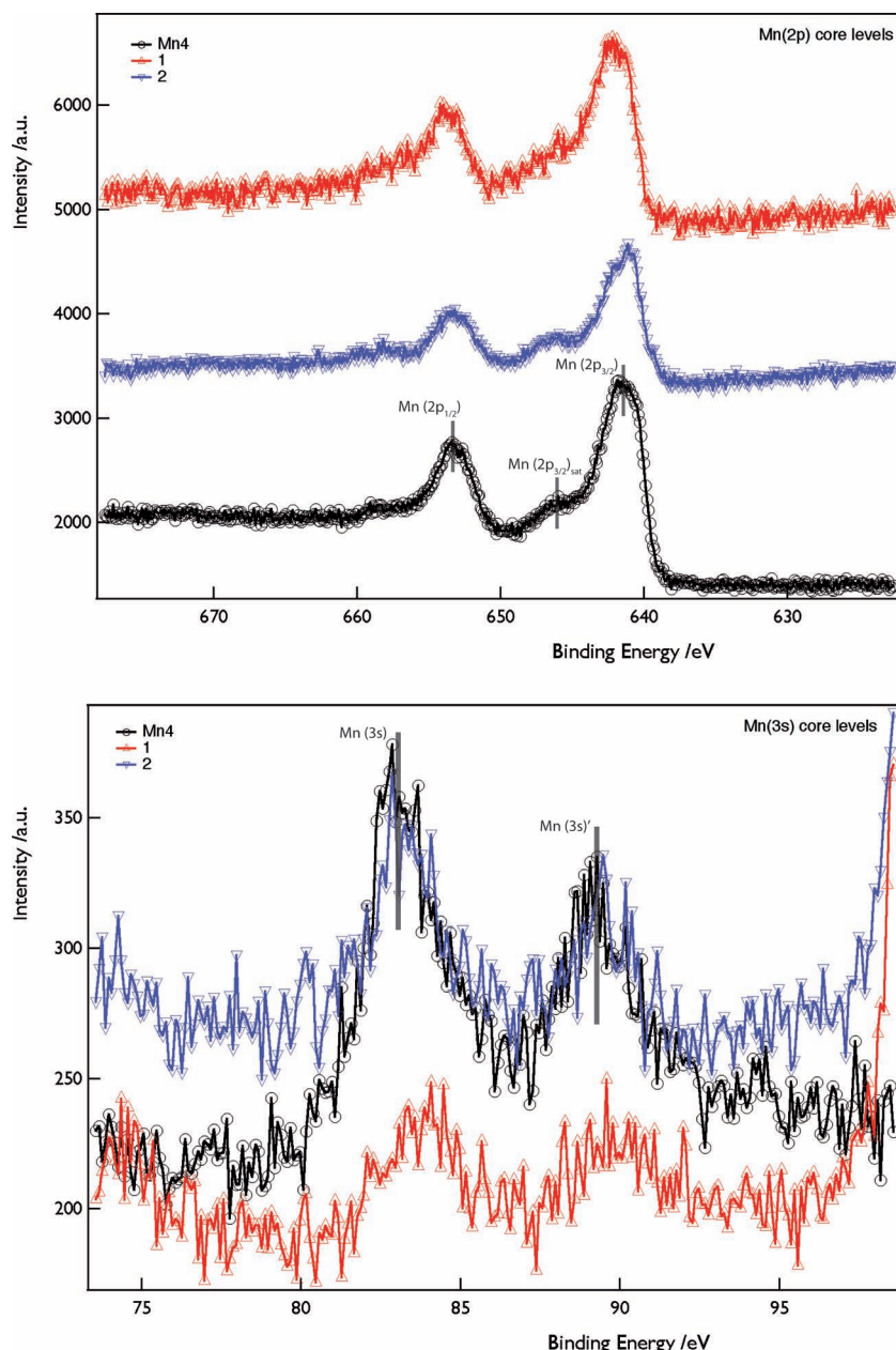
Figure 5. Core-level Mn 2p (top) and 3s (bottom) XPS spectra of the bulk \text{Mn}_4 complex (black circles) and the \text{Mn}_4 -MWNTs hybrids (1: red triangles and 2: blue inverted triangles).
